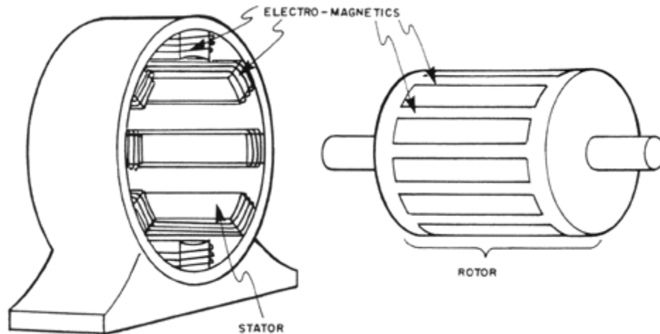
Reliance Electric's diagram of an AC motor, showing the "stator" and "rotor" components.
